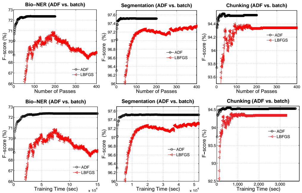
Figure 4 Comparisons between the ADF method and the batch training method LBFBS. (Top Row) Comparisons based on training passes. As we can see, the ADF method converges much faster than the LBFBS method, and with better accuracy on the convergence state. (Bottom Row) Comparisons based on wall-clock time.
